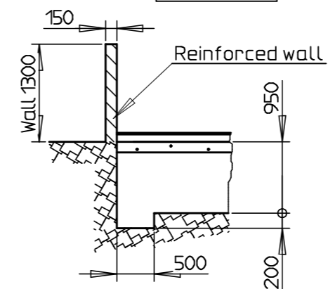
Section B-B
